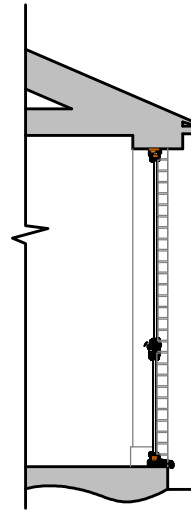
Window Section @ 1/50
