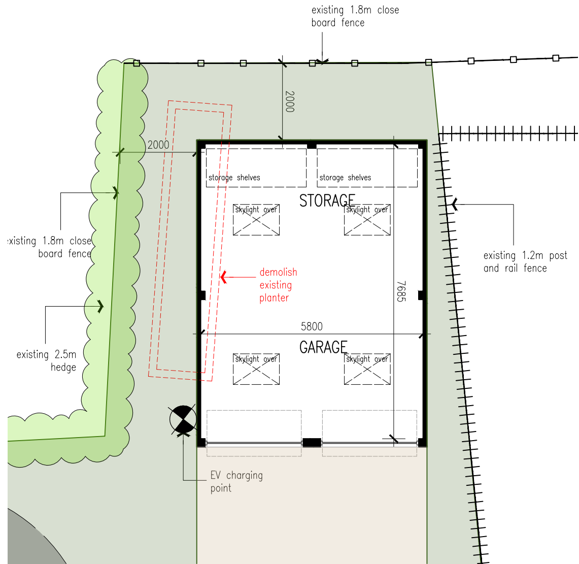
[01] GARAGE 2 PLAN
