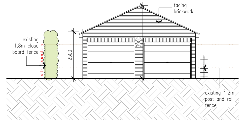
[03] GARAGE 2 FRONT ELEVATION (SOUTH EAST)
