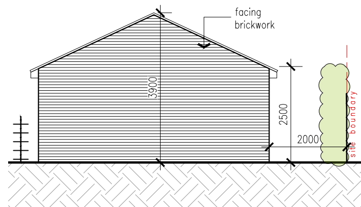
[05] GARAGE 2 REAR ELEVATION (NORTH WEST)
