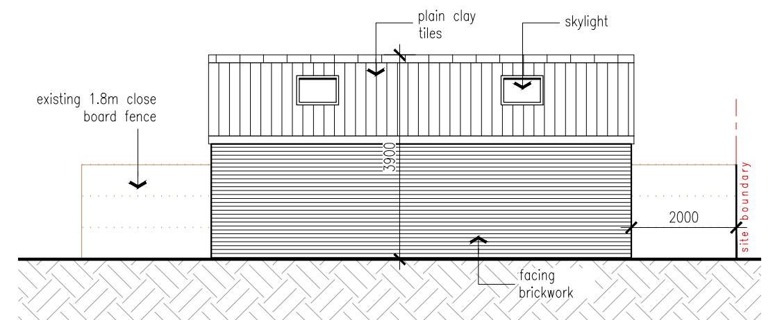
[06] GARAGE 2 SIDE ELEVATION (NORTH EAST)
