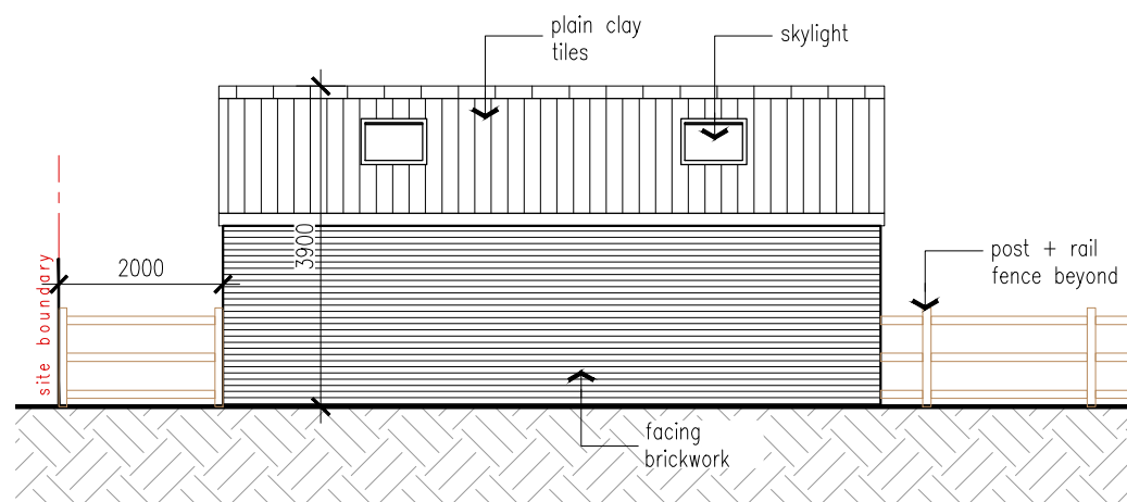
[04] GARAGE 2 SIDE ELEVATION (SOUTH WEST)
