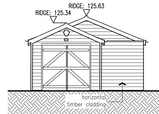
[03] BUILDING G - SOUTH WEST ELEVATION
