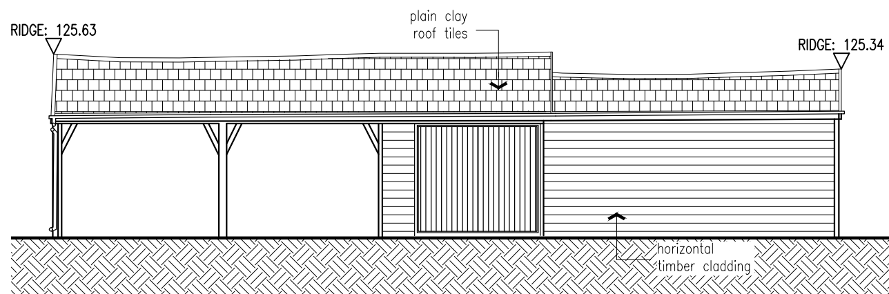
[02] BUILDING G - NORTH WEST ELEVATION
