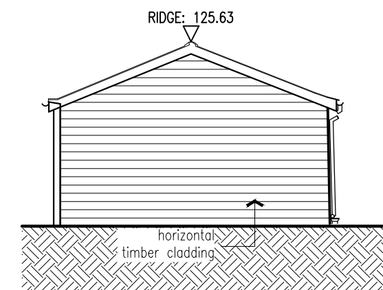
[05] BUILDING G - NORTH EAST ELEVATION
