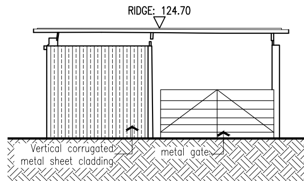
[02] BUILDING D - NORTH EAST ELEVATION
