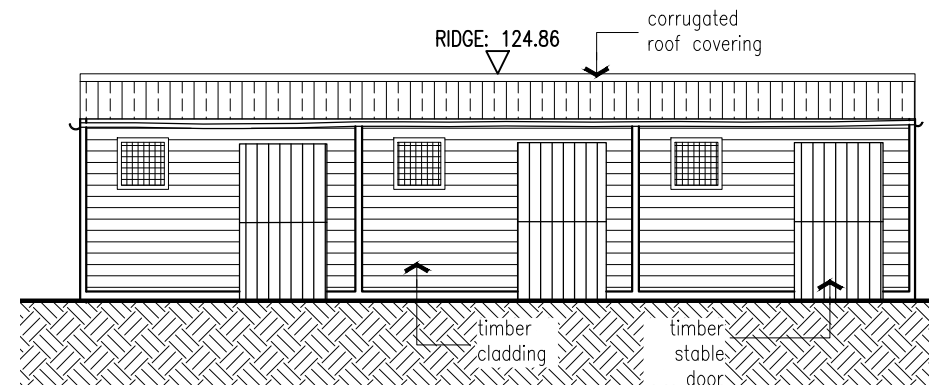
[07] BUILDING E - WEST ELEVATION
