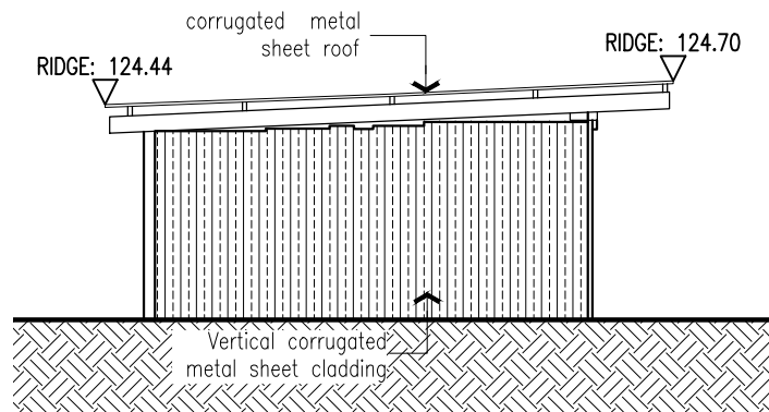
[03] BUILDING D - SOUTH EAST ELEVATION
