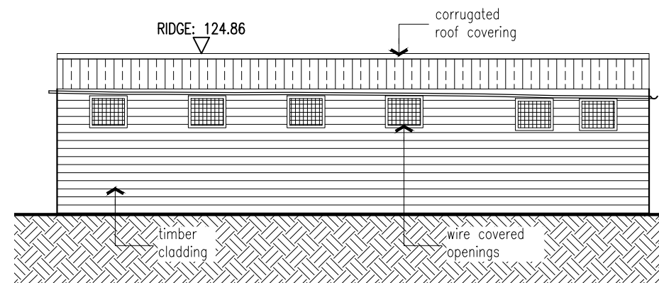
[09] BUILDING E - EAST ELEVATION
