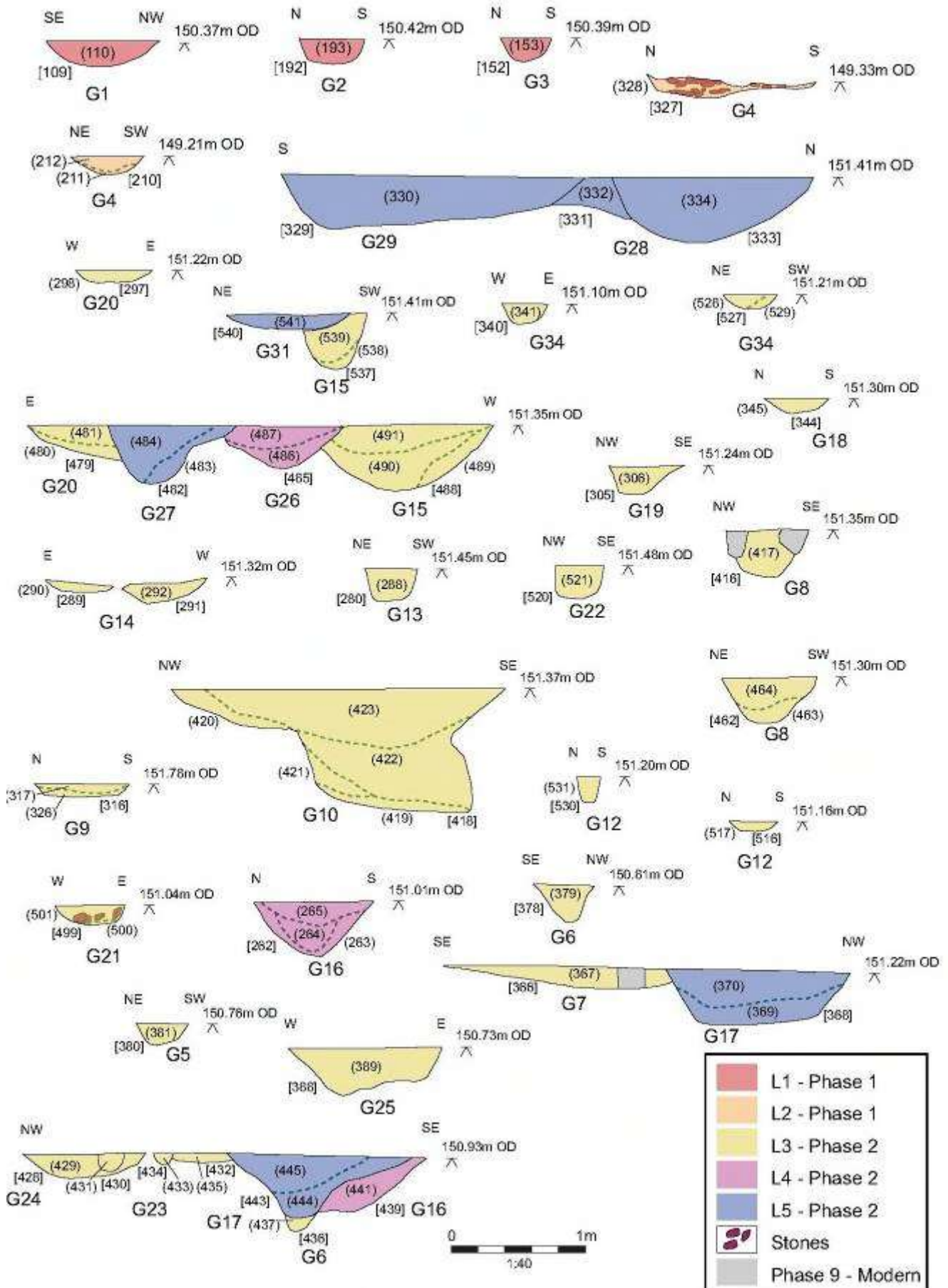
Figure 8: Selected section drawings from Phase 1, late Bronze Age/early Iron Age and Phase 2, Iron Age
