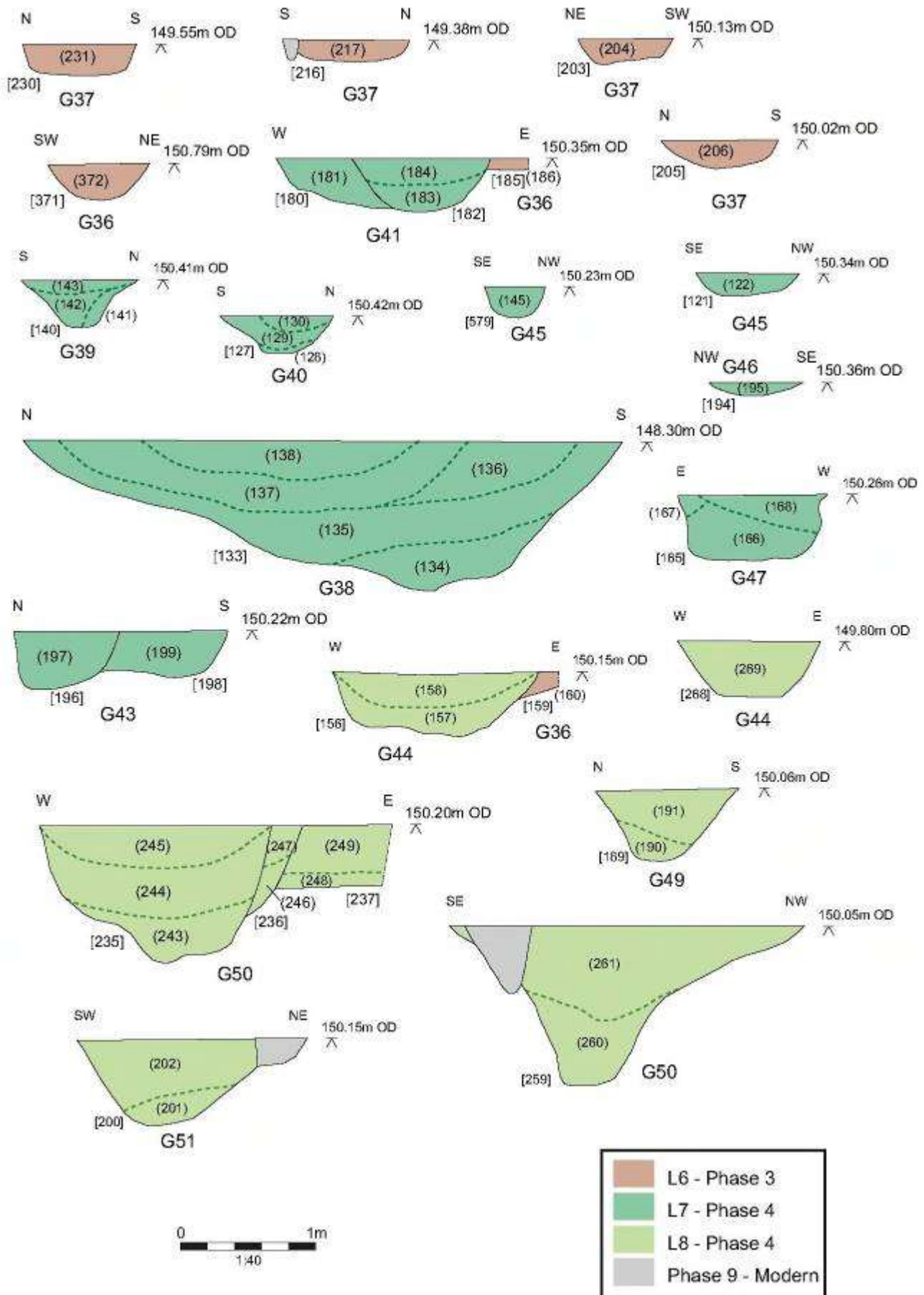
Figure 9: Selected section drawings from Phase 3, undated and Phase 4, medieval
