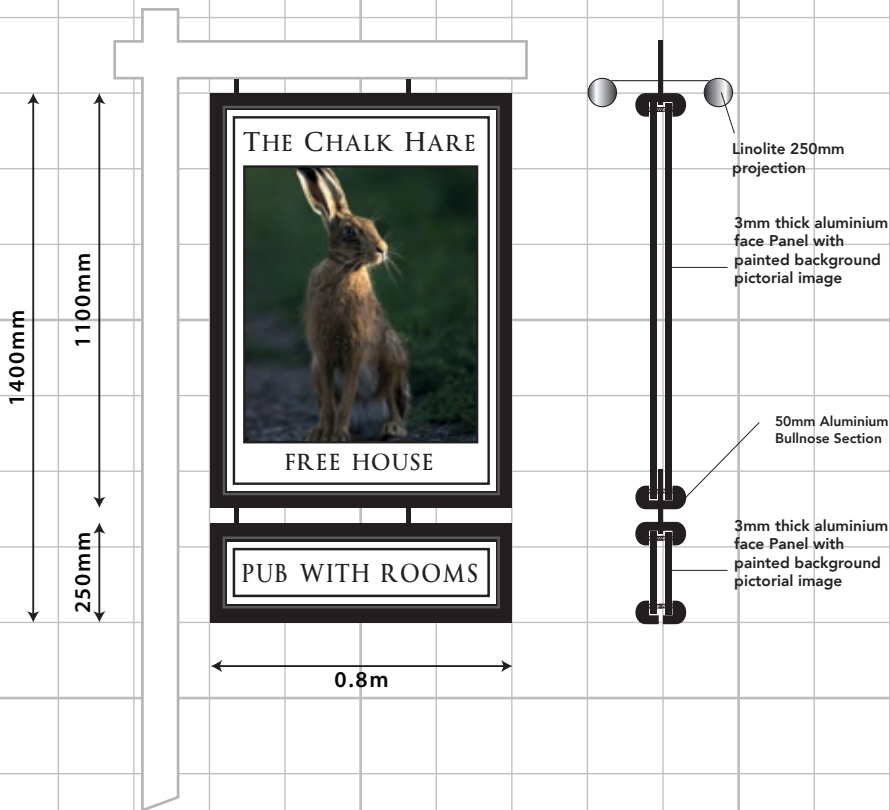
A ONE X NEW PICTORIAL TO A NEW GALLOW STYLE BRACKET AND DROP PANEL AND LINOLITES, CLAMPED TO WALL SIZE. 0.8m x 1400mm. H.A.G. 2.5m.
