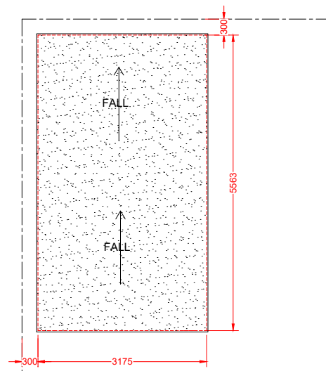
ROOF FLOOR PLAN
