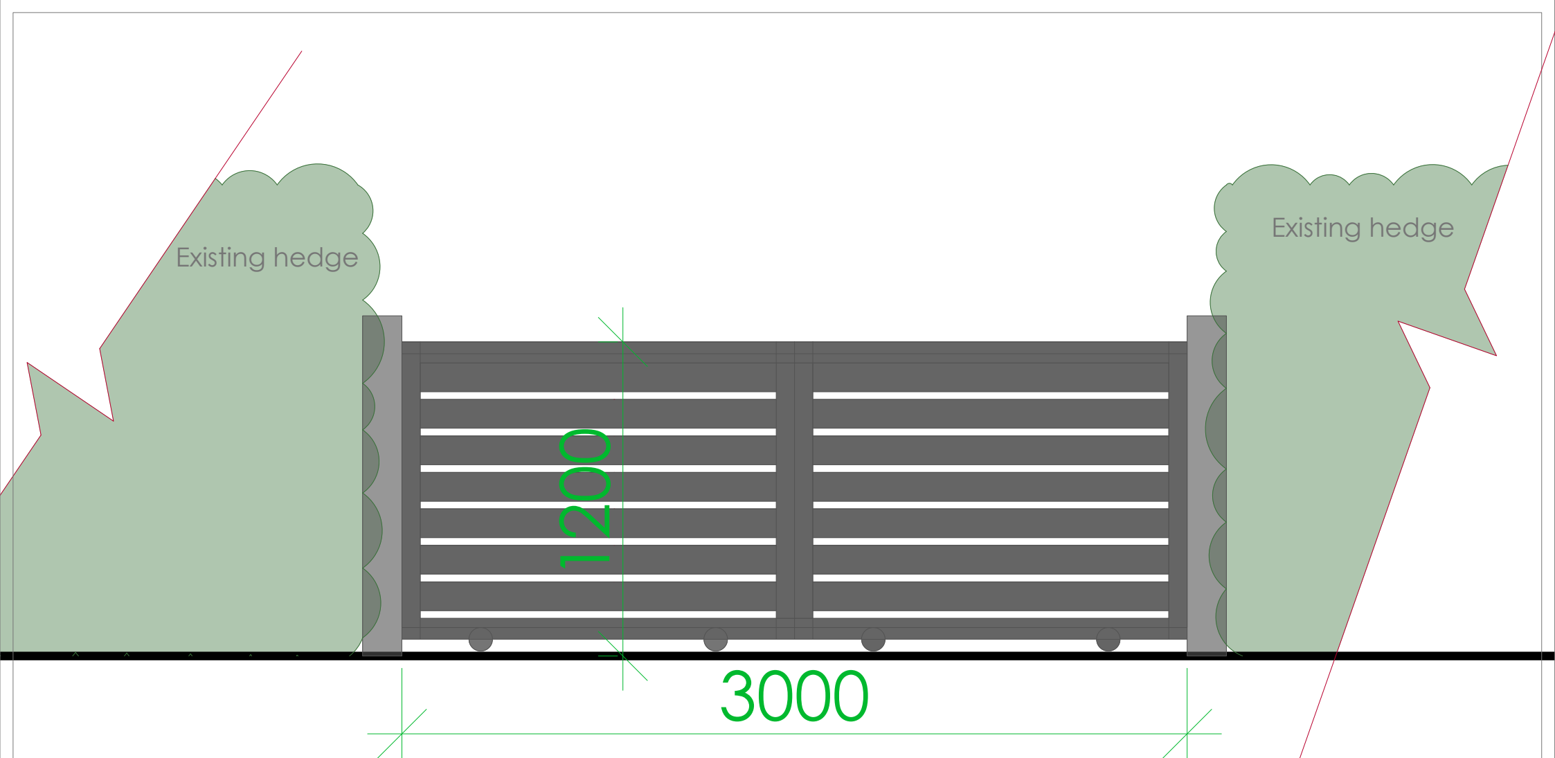
Sliding aluminium driveway gate.
