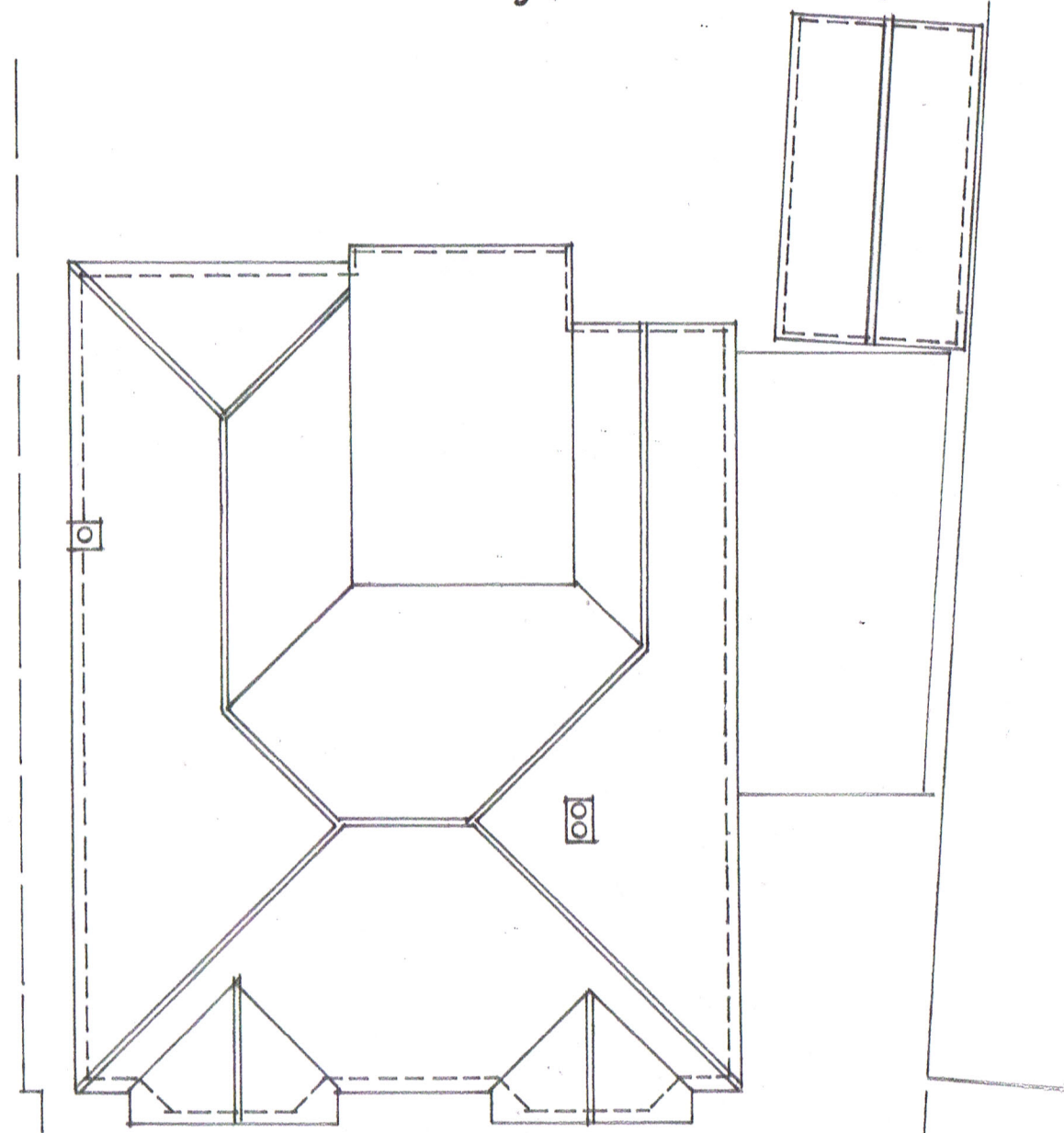
ROOF PLAN
