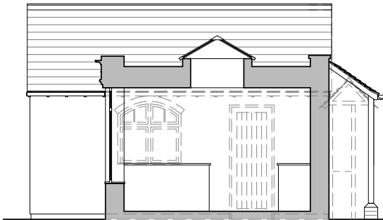
Proposed garage side (northeast) elevation
