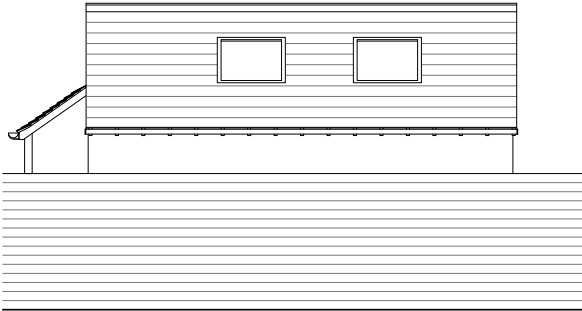
Proposed garage side (southwest) elevation
