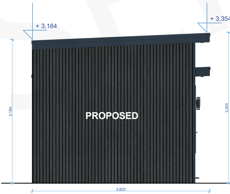
LEFT VIEW
