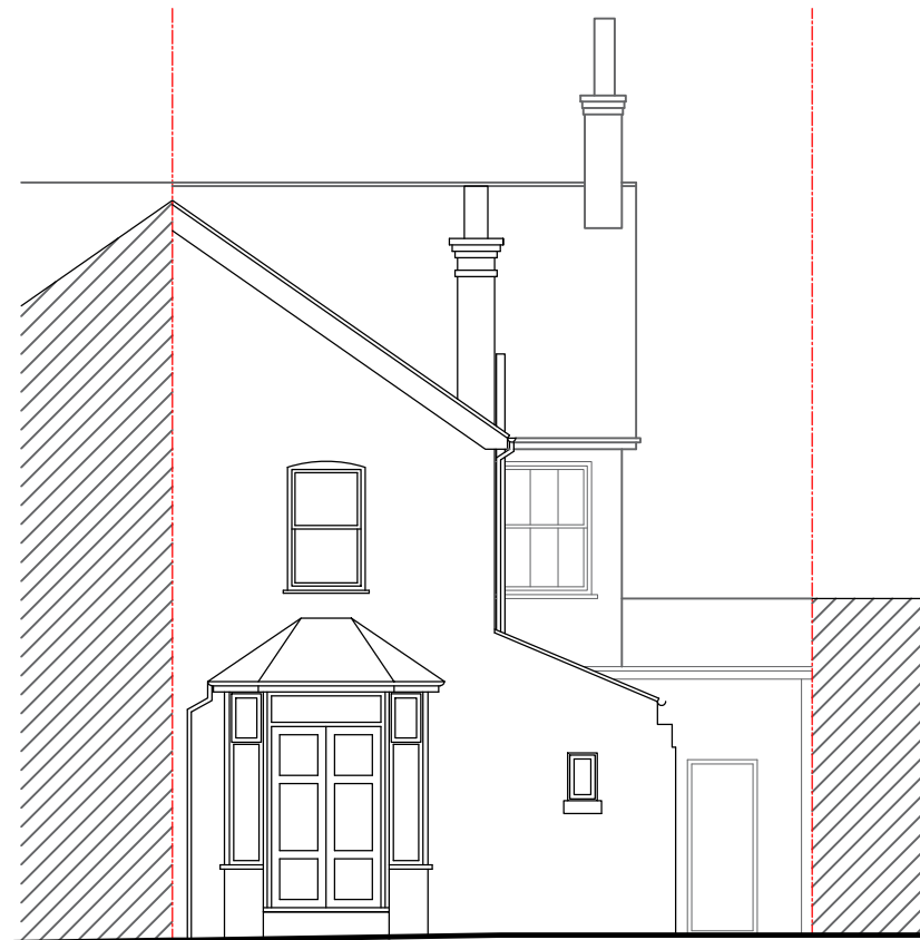
Rear Elevation @ 1/100
