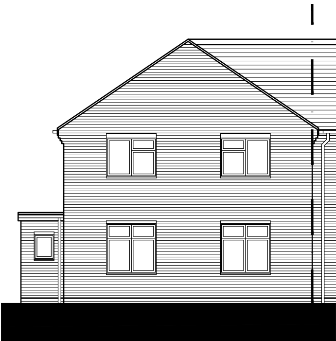
SIDE ELEVATION (D-D)
