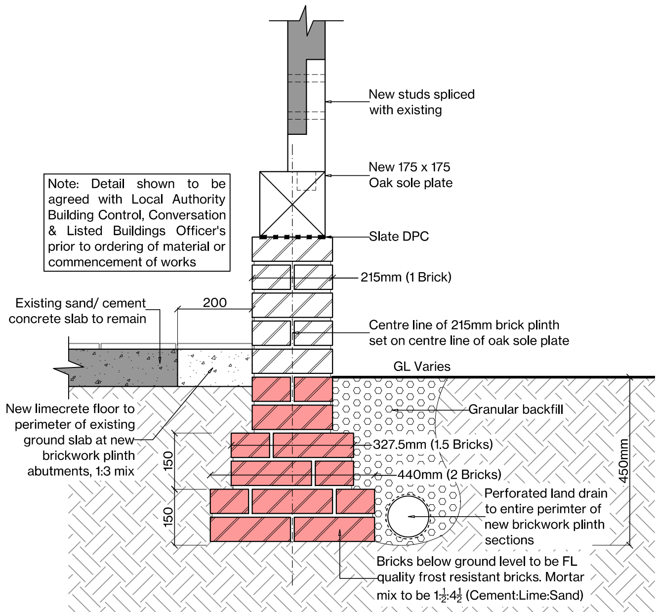
Replacement Plinth Detail 1:10
