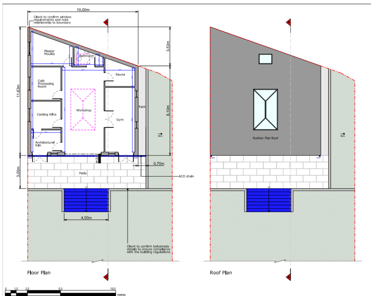
Figure 5.1 – Proposed Layout
