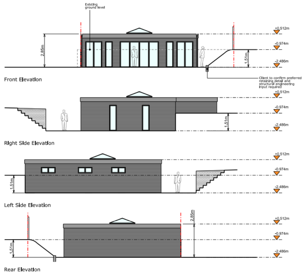
Figure 5.1.1 – Proposed Elevations
