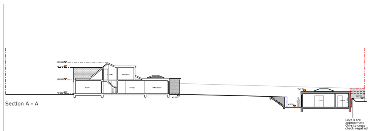
Figure 5.1.2 – Proposed Sectional Drawing
