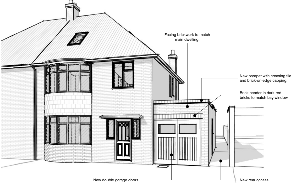
4 Front View - Proposed @A3
