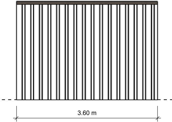
South Elevation
