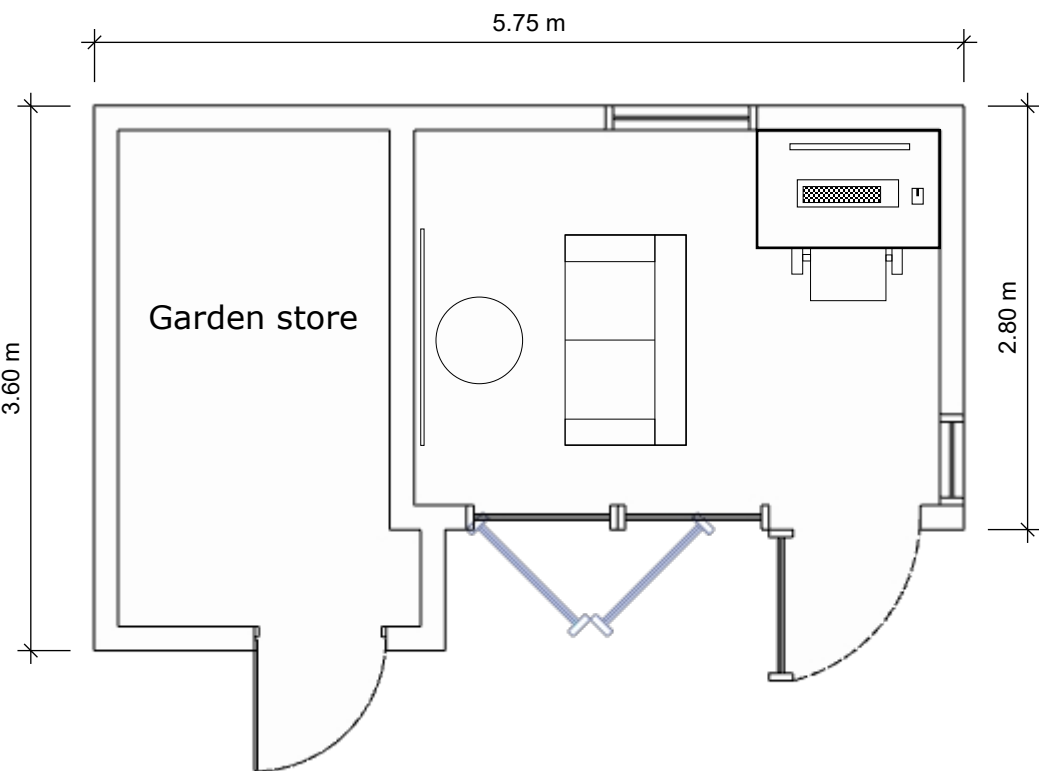
Floor Plan
