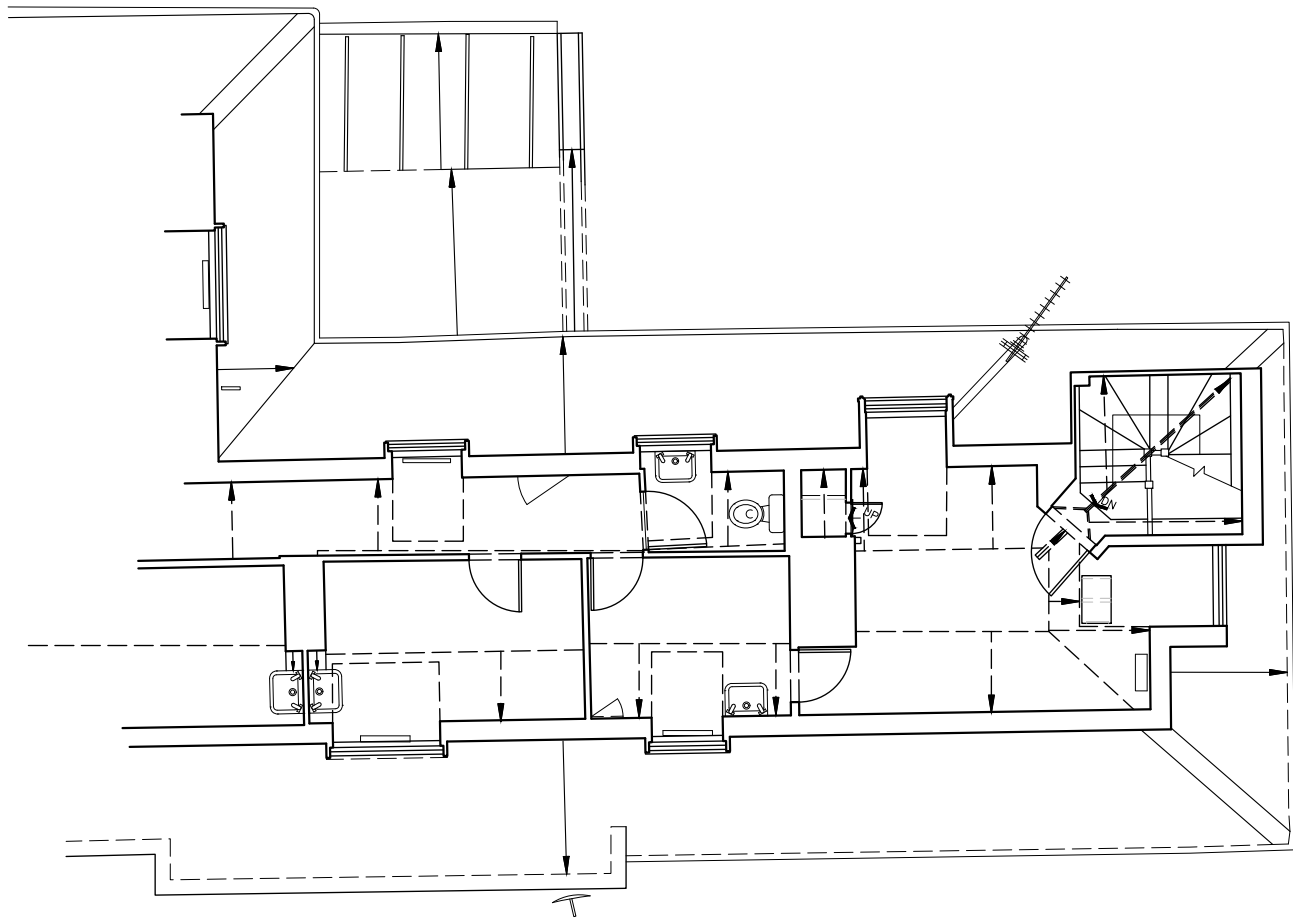
B Main Building, Level 01 02050
