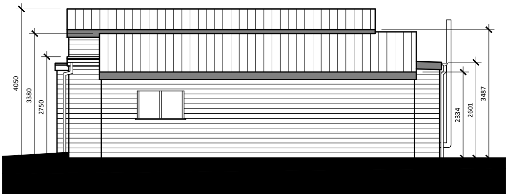
SIDE ELEVATION (D-D)
