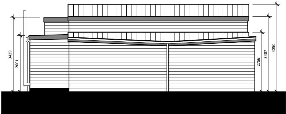
SIDE ELEVATION (B-B)
