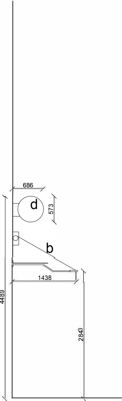
Canopy section as proposed
