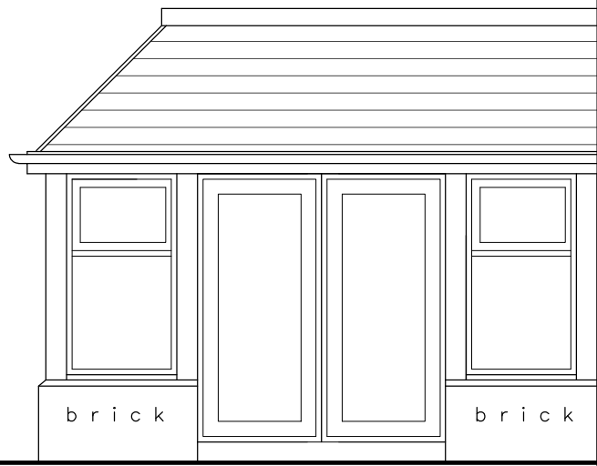
Side Elevation @ 1/50
