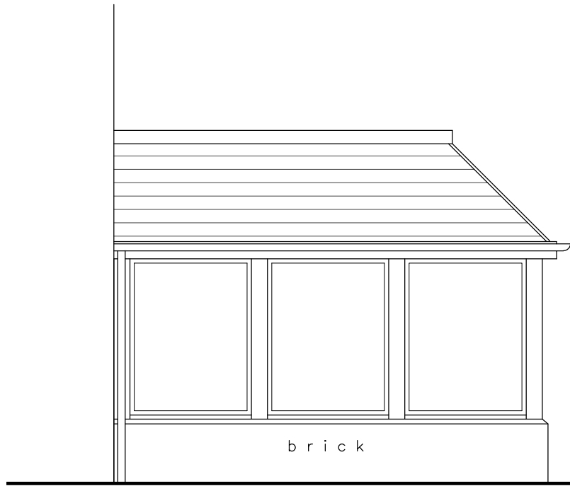
Side Elevation @ 1/50
