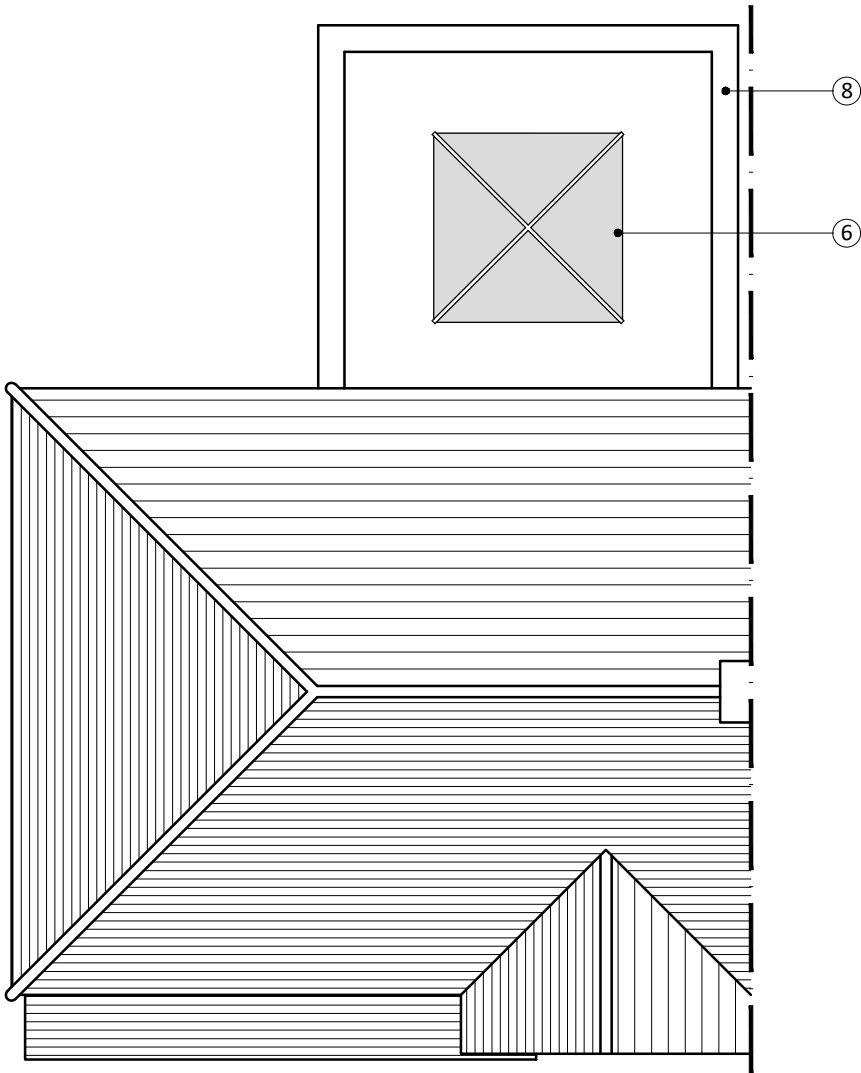
ROOF PLAN
