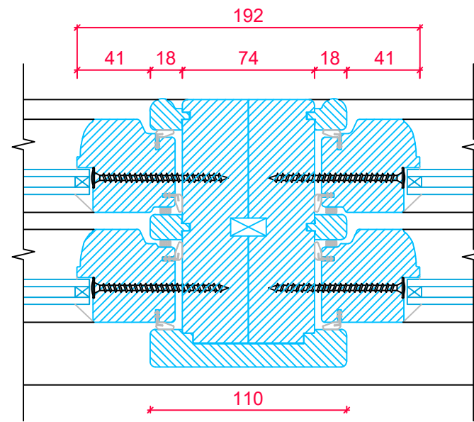
CENTRAL MULLION FOR DOUBLE FIXED SASH
