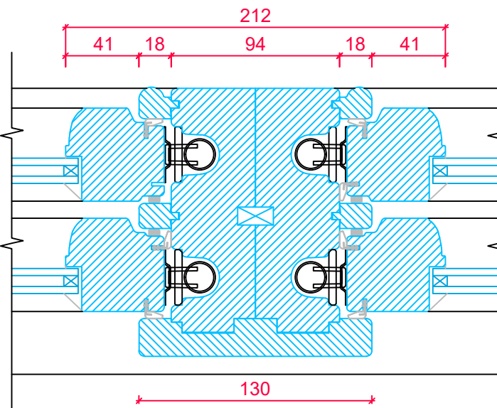
CENTRAL MULLION FOR DOUBLE OPENING SASH (both sashes open independently)
