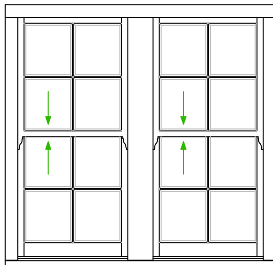
TYPICAL DOUBLE OPENING SASH LAYOUT
