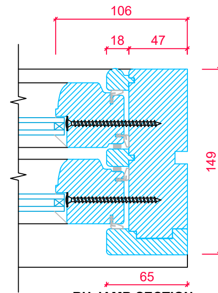
RH JAMB SECTION FOR FIXED SASH (LH IS DIRECT MIRROR)
