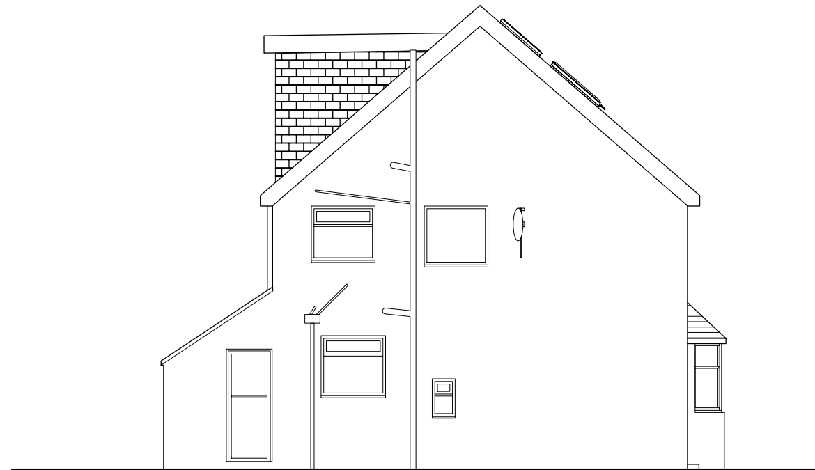
2. Side (north-east) Elevation 1:100
