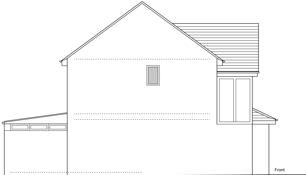
2 26 Gibson Close Existing Side/North East Elevation 1:100
