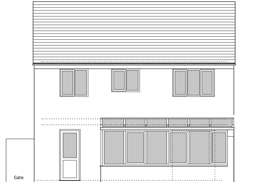
3 26 Gibson Close Existing Rear Elevation 1:100
