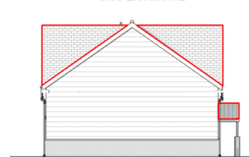
Side Elevation W
