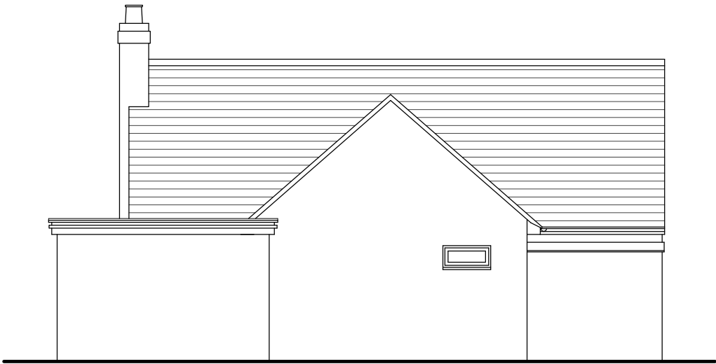
Front Elevation @ 1/100
