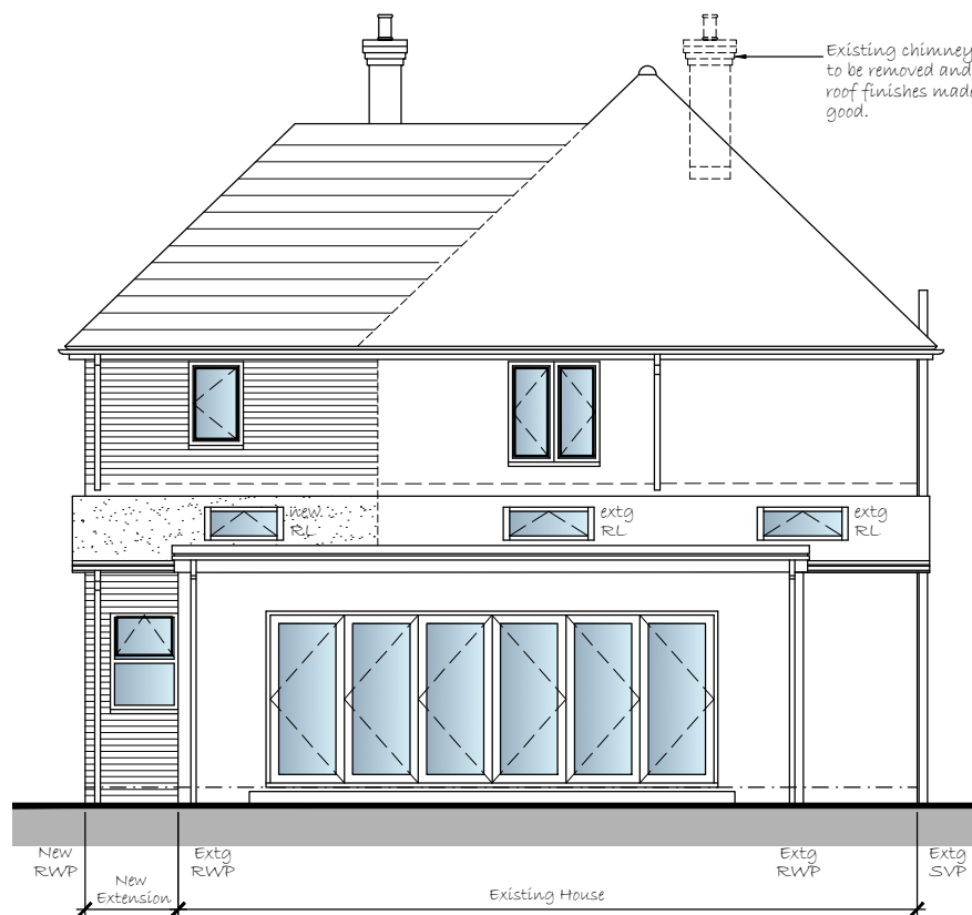
Rear (north) Elevation @ 1:100
