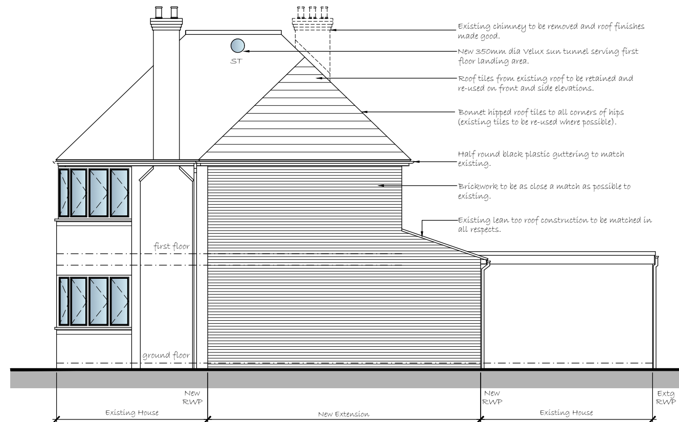
Side (east) Elevation @ 1:100
