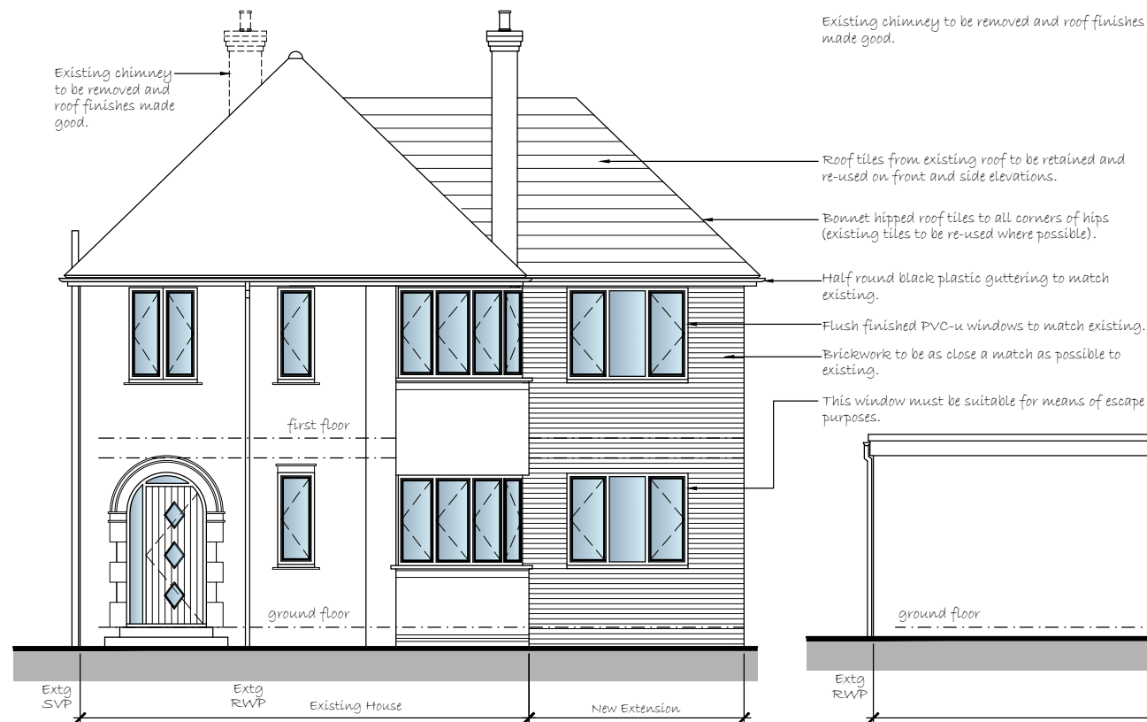
Front (south) Elevation @ 1:100
