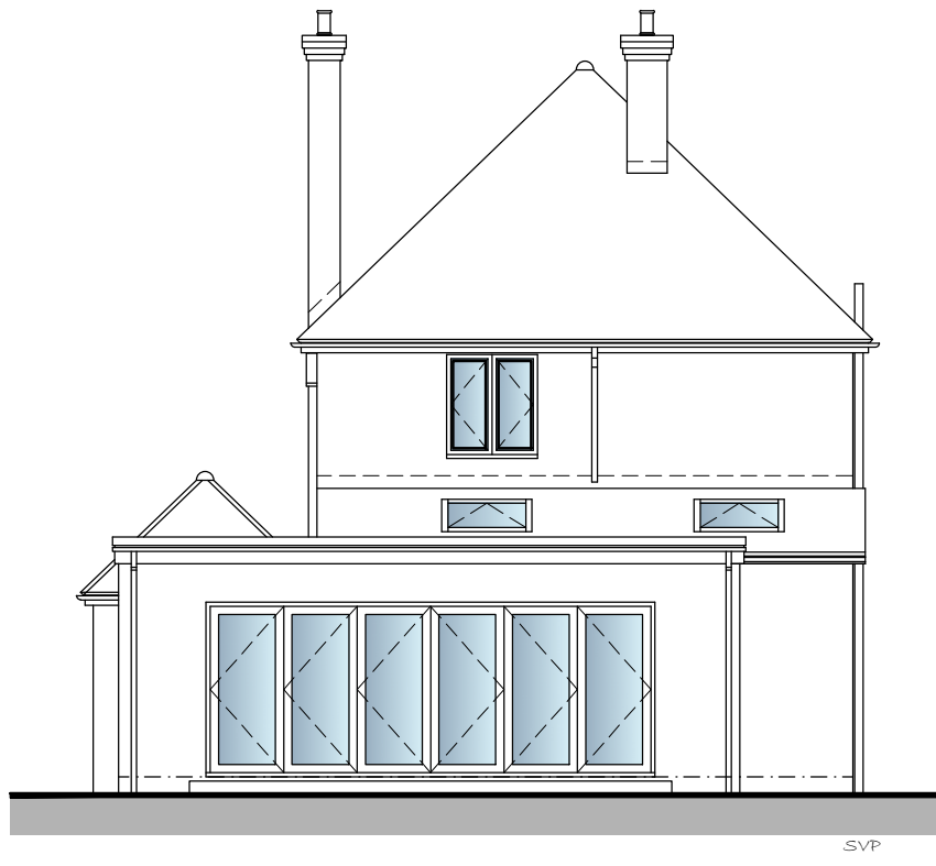
Rear (north) Elevation @ 1:100
