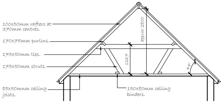
Cut Roof Section A-A @ 1:100
