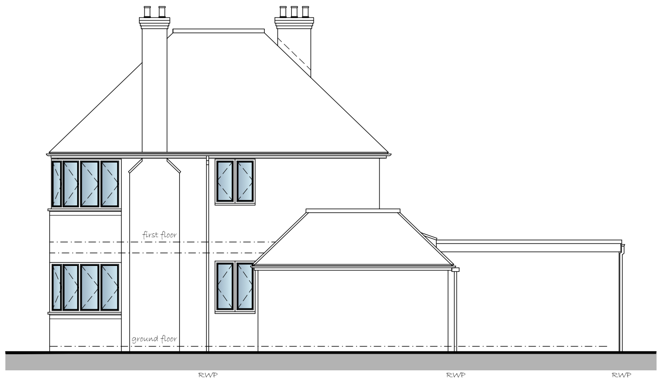
Side (east) Elevation @ 1:100
