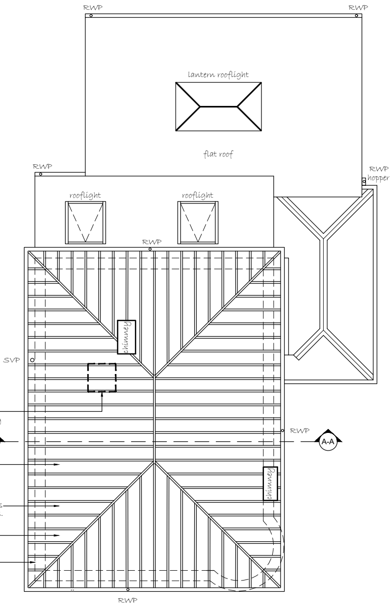
Roof Space Plan @ 1:100
