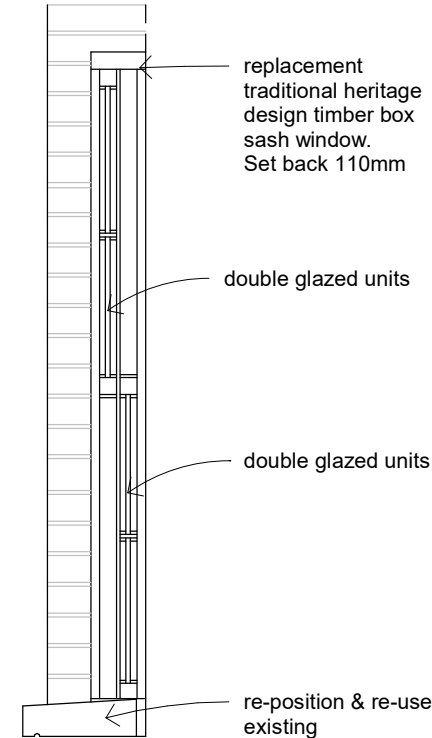
Section
