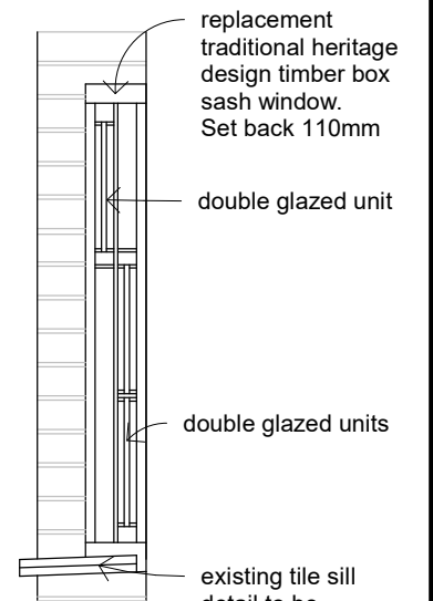
Section
