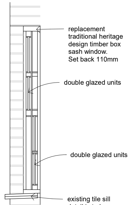
Section
