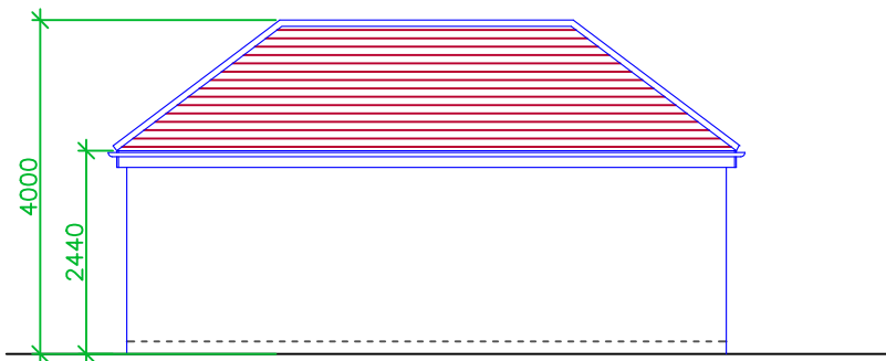
EAST ELEVATION AS PROPOSED
