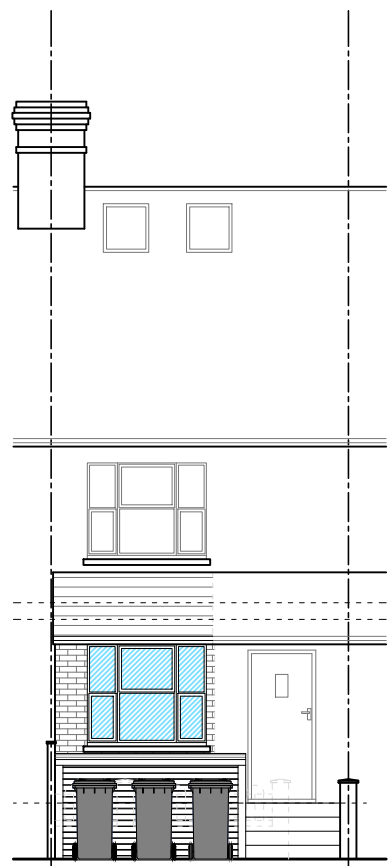
FRONT ELEVATION
