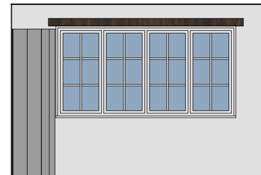
E-04 Southeast Elevation 1:50
