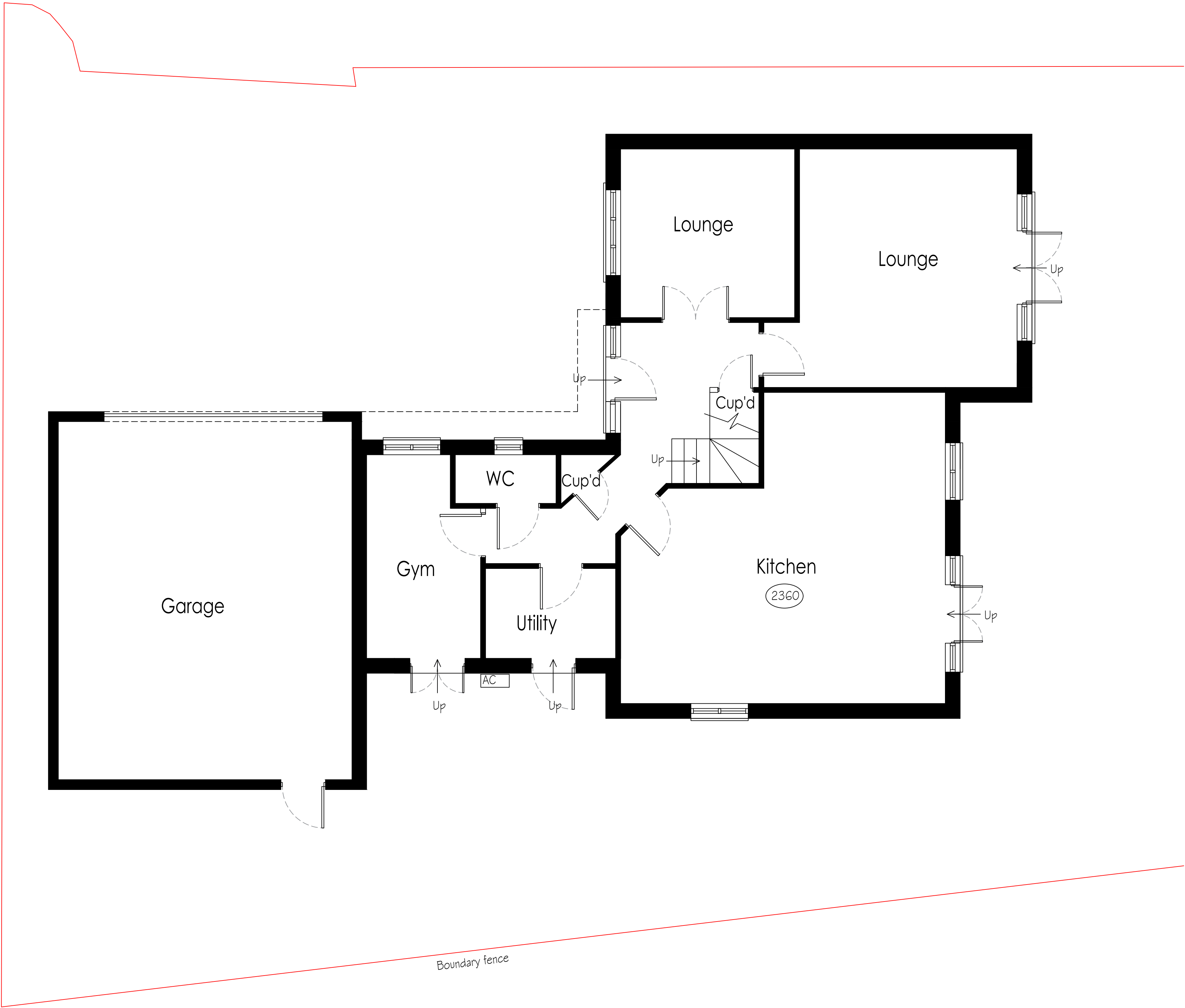
EXISTING GF PLAN @1:50 @ A1
