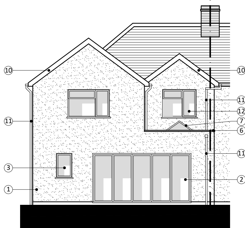
REAR ELEVATION (B-B)
