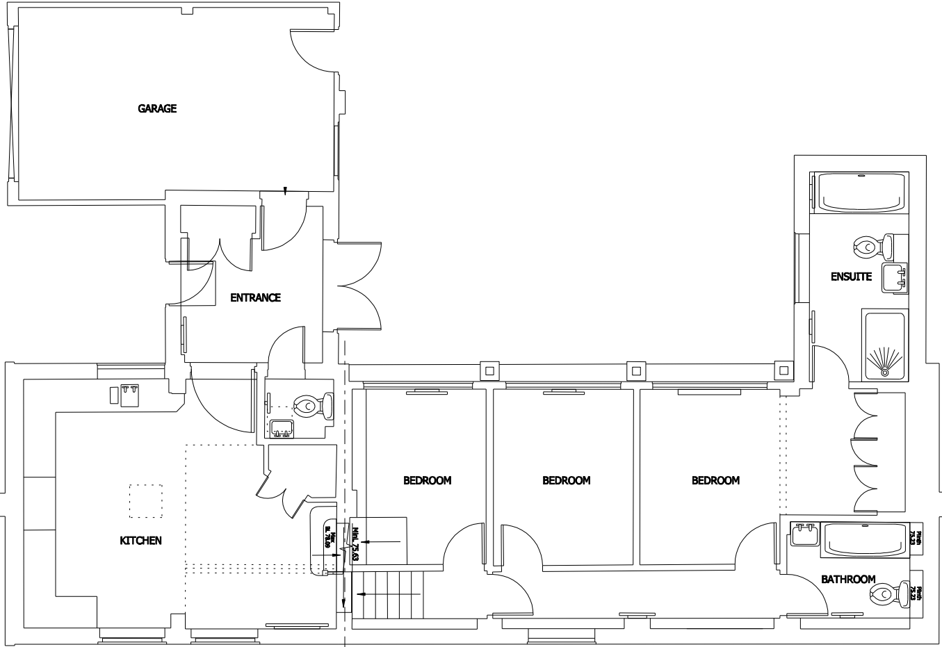
GROUND FLOOR (0)
