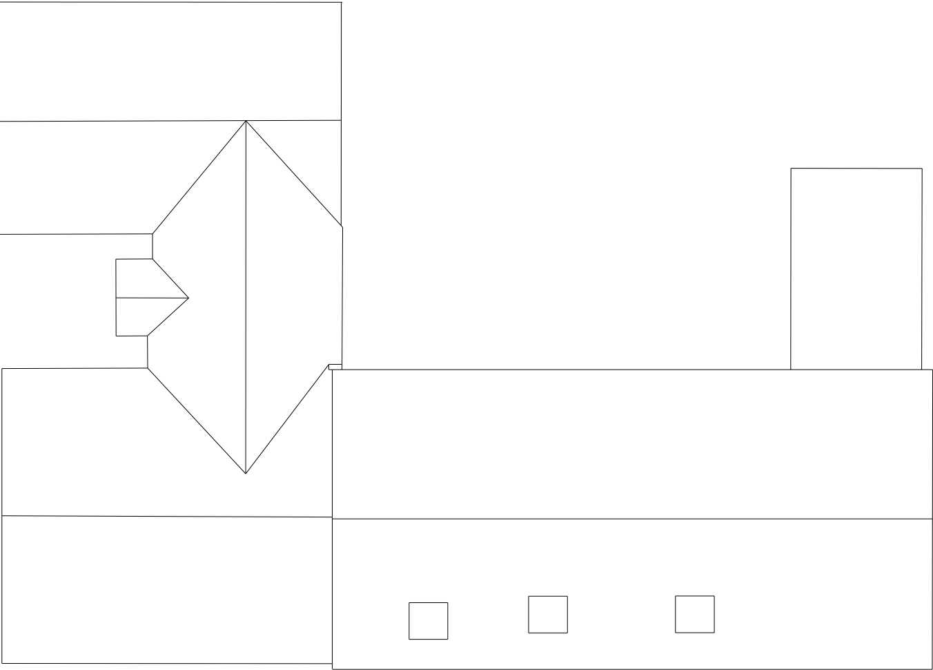
ROOF
