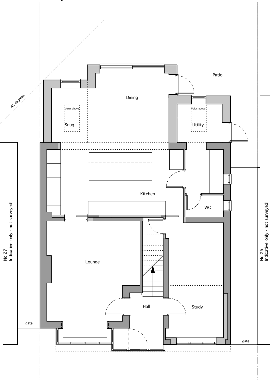
1 26 Gibson Close Proposed Ground Floor Plan 1:100
