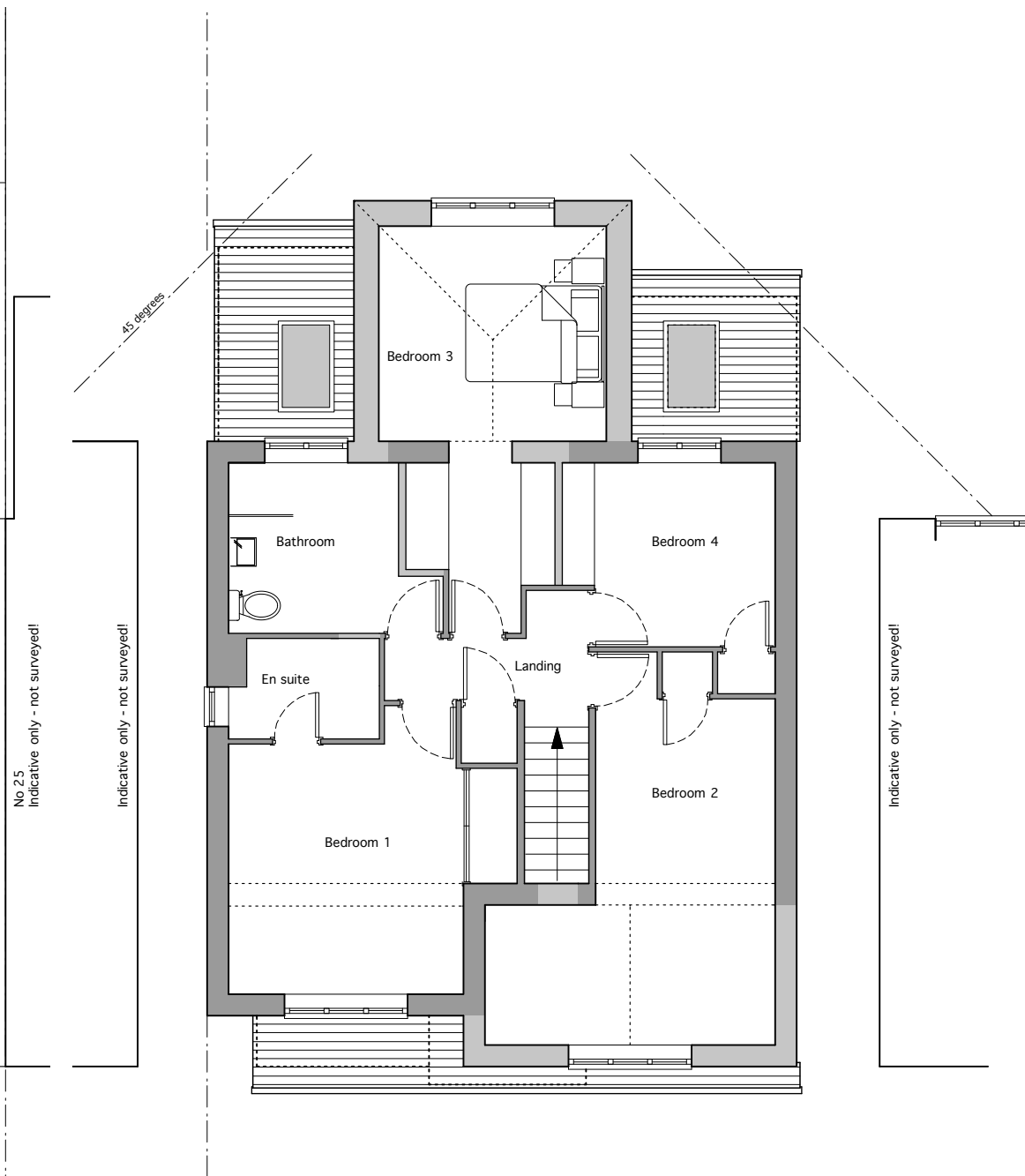
2 26 Gibson Close Proposed 1.Floor Plan 1:100
