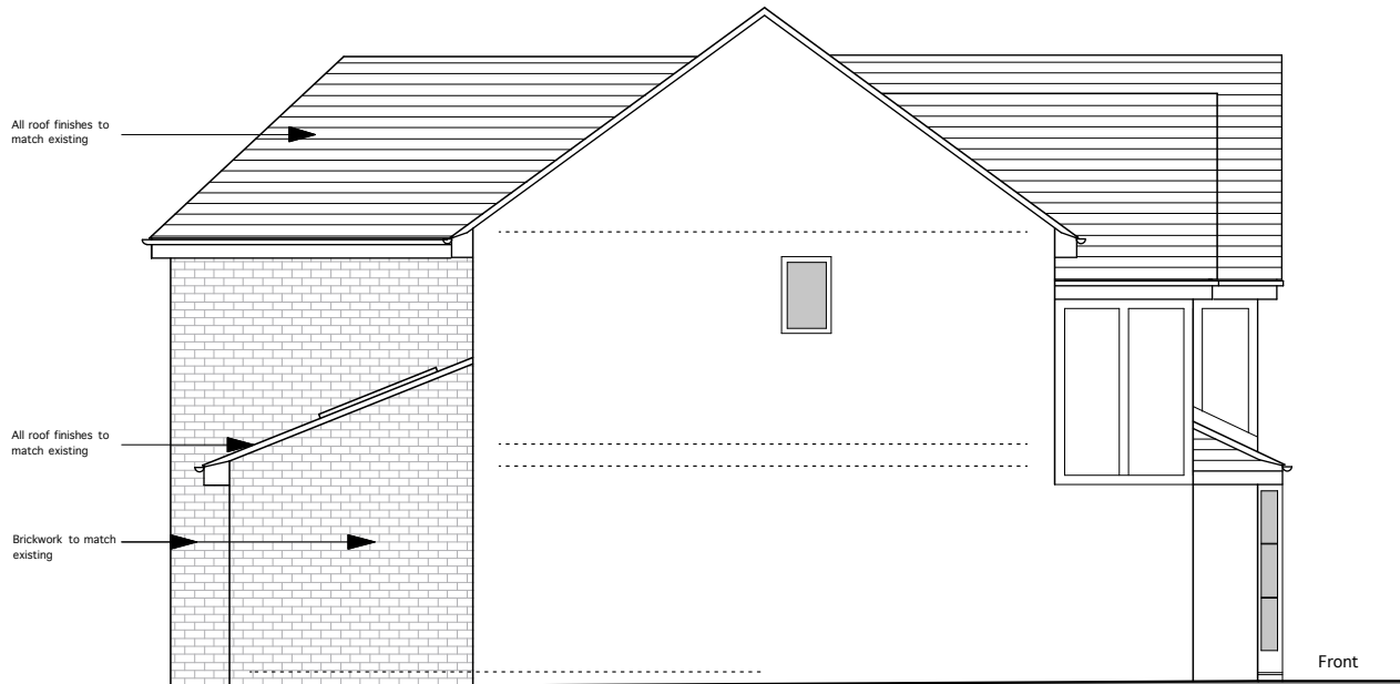
2 26 Gibson Close Proposed Side/North-East Elevation 1:100
