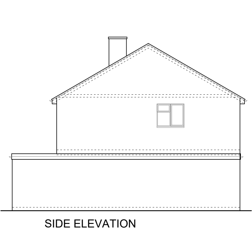
SIDE ELEVATION
