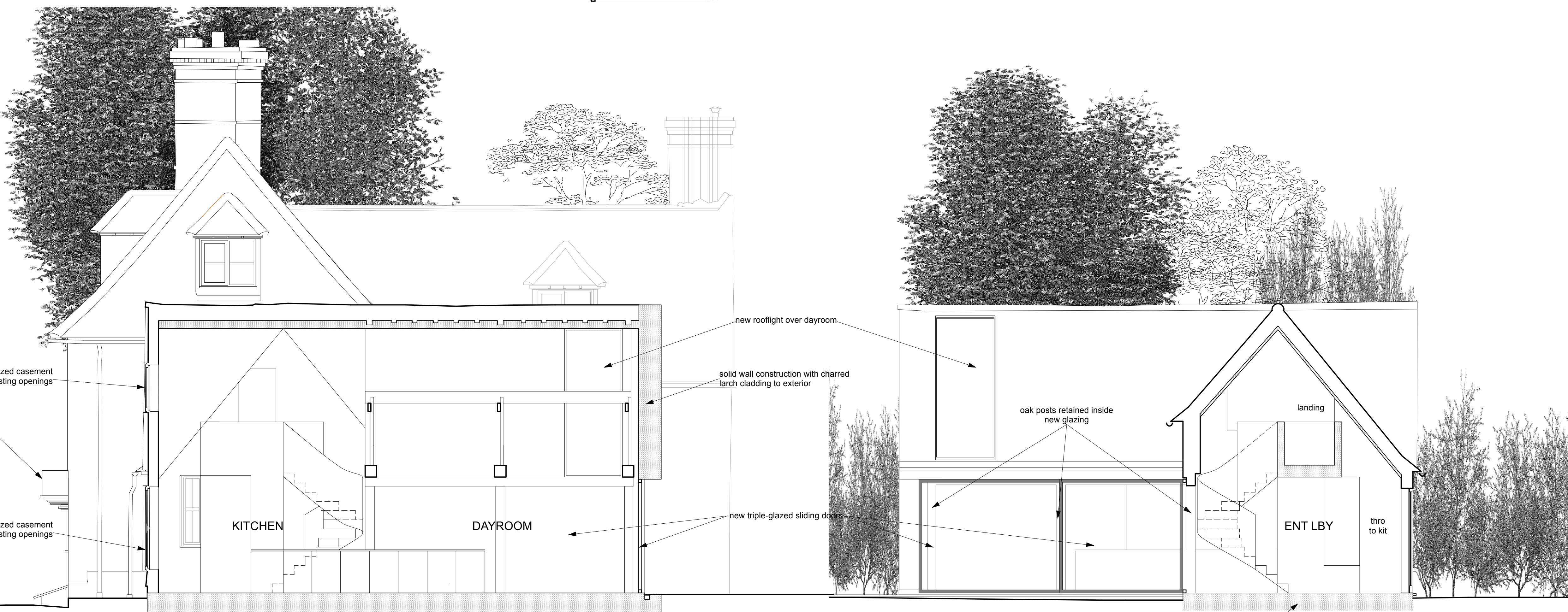
SECTION xx AS PROPOSED
