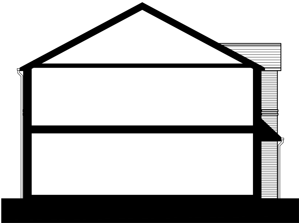
SIDE ELEVATION (B-B)
