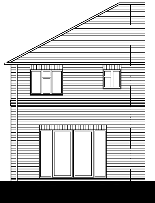
REAR ELEVATION (C-C)
