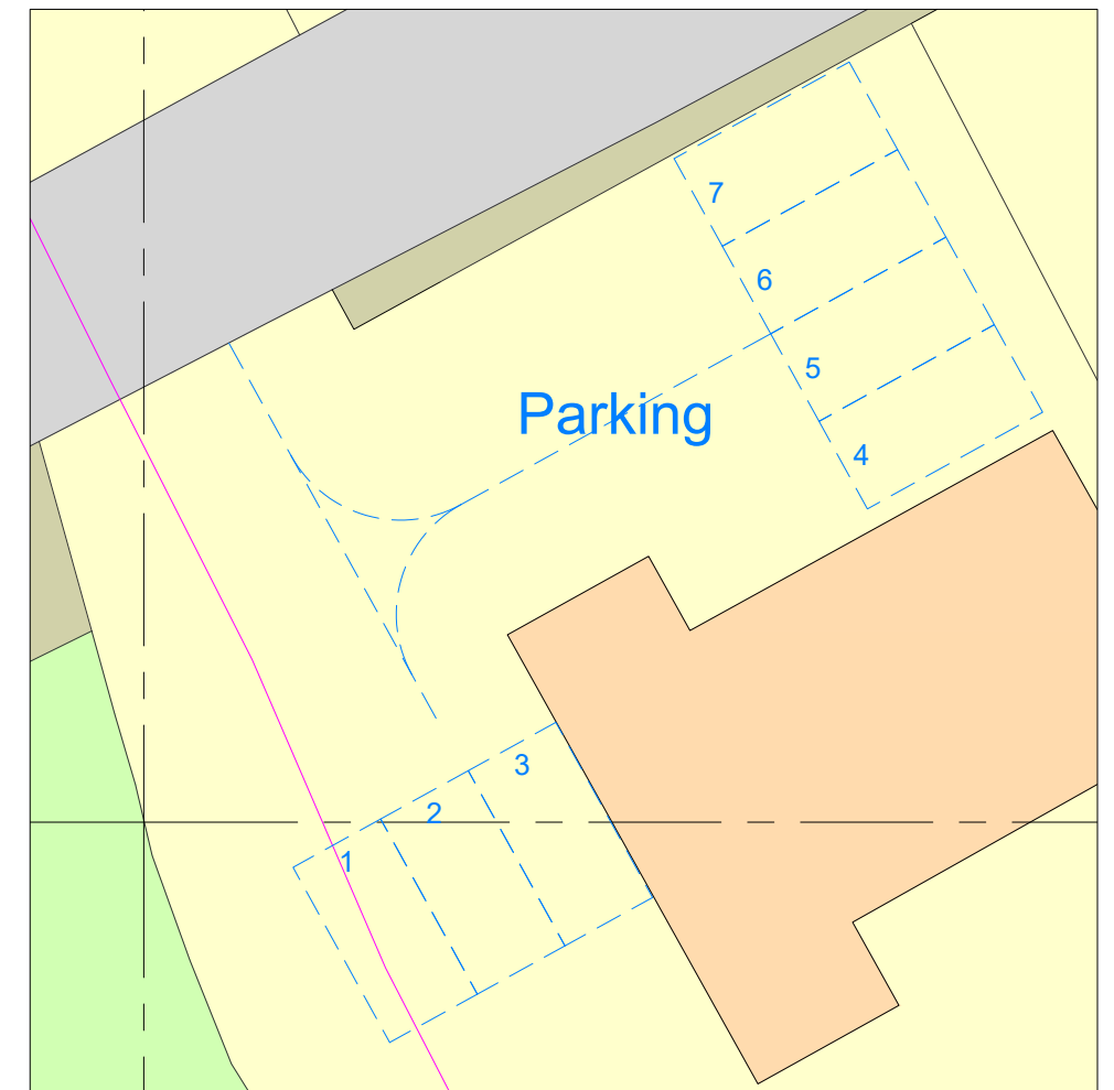
PARKING PLAN 1:200
