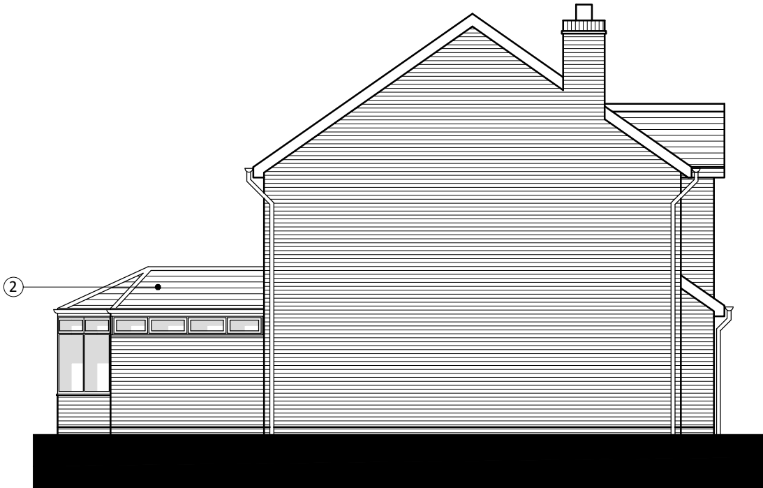
SIDE ELEVATION (B-B)
