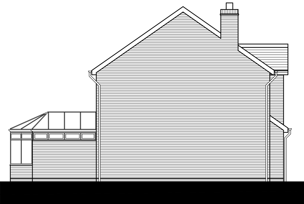
SIDE ELEVATION (B-B)
