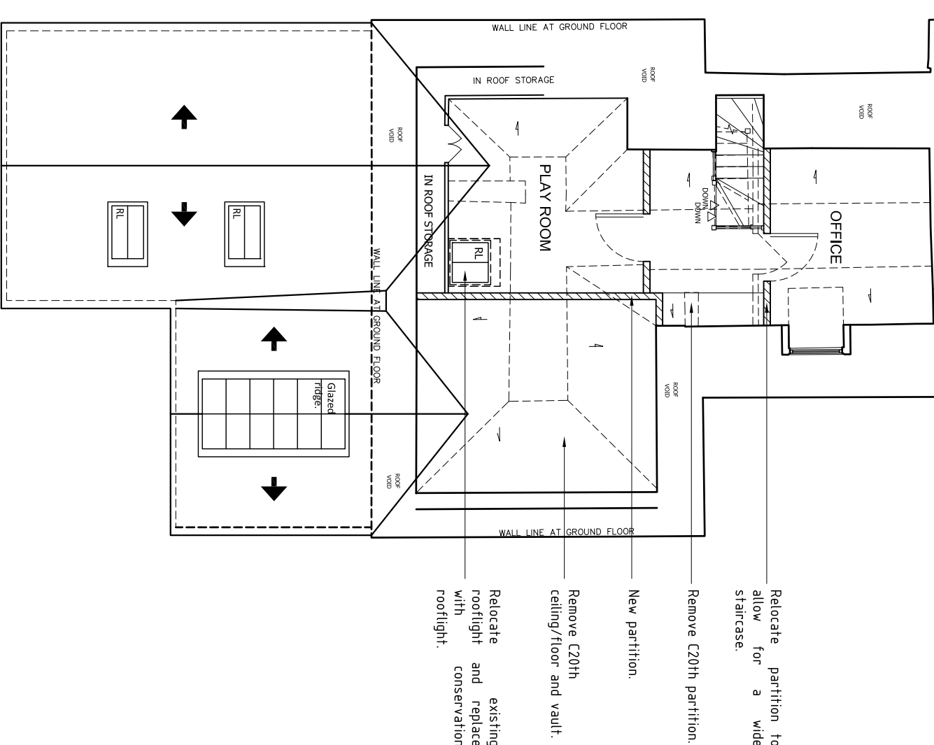
SECOND FLOOR LAYOUT
