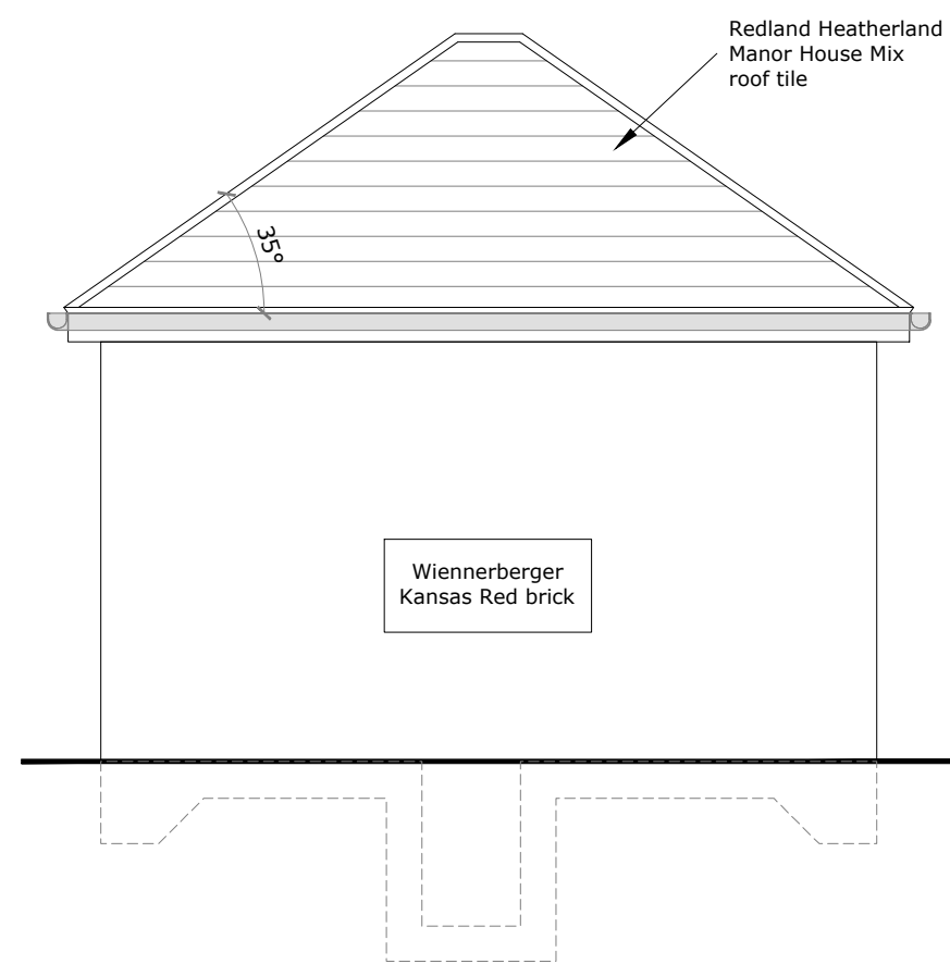
Elevation C
