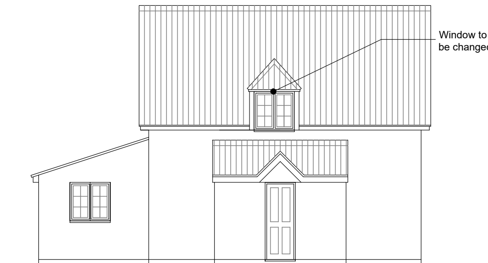
Side Elevation
