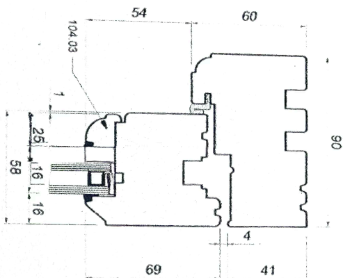
Attachment 4: vertical section drawing
