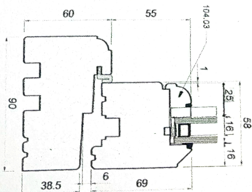
Attachment 4: vertical section drawing
